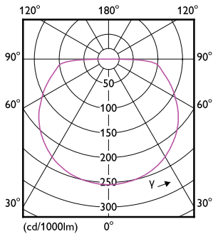
Light Distribution Diagram - LS161 COB LED12 13W 940 5M 24V
