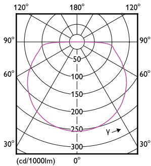
Light Distribution Diagram - LS161 COB LED8 8.5W 940 5M 24V
