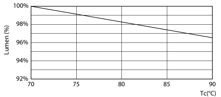
Lumen Maintenance Diagram - MAS LEDtube 1200mm HO 26W 840 G5 VWV BR
