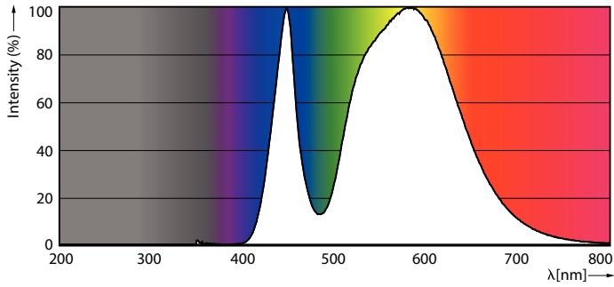
Spectral Power Distribution Colour - MAS LEDtube 1200mm HO 26W 840 G5 VWV BR
