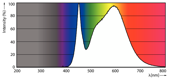
Spectral Power Distribution Colour - LEDBulb 11W E27 4000K W 1PF/40 BR
