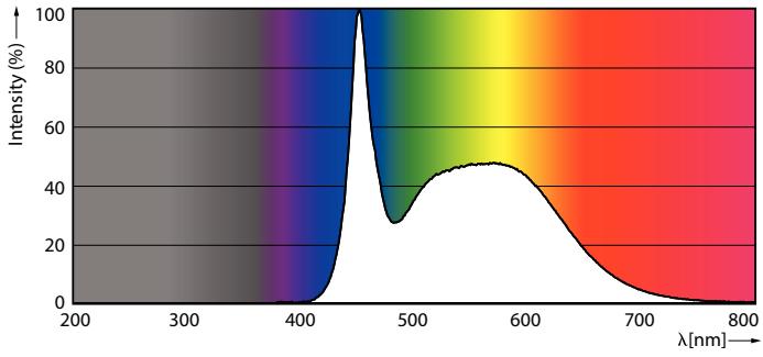
Spectral Power Distribution Colour - LEDBulb 13W E27 6500K W 1PF/40 BR
