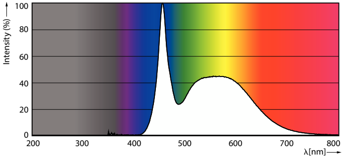
Spectral Power Distribution Colour - LEDGlobe13-175W G95 E27 CDL100-240V BR
