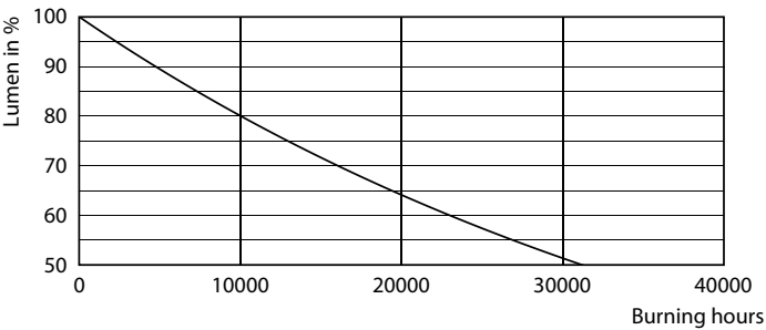
Lumen Maintenance Diagram - LEDGlobe13-175W G95 E27 CDL100-240V BR
