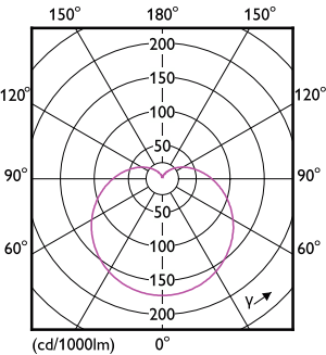
Light Distribution Diagram - LEDGlobe13-175W G95 E27 CDL100-240V BR
