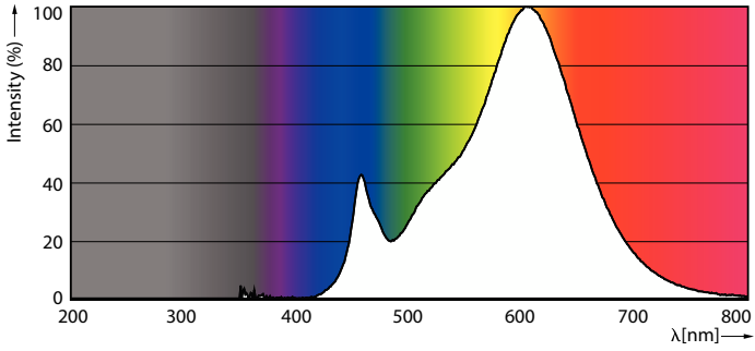
Spectral Power Distribution Colour - LEDGlobe13-175W G95 E27 WW 100-240V BR
