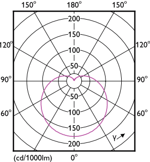
Light Distribution Diagram - LEDGlobe13-175W G95 E27 WW 100-240V BR
