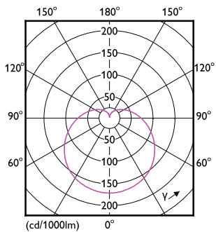
Light Distribution Diagram - LEDBulb 18W E27 6500K W A70 1PF/6 BR
