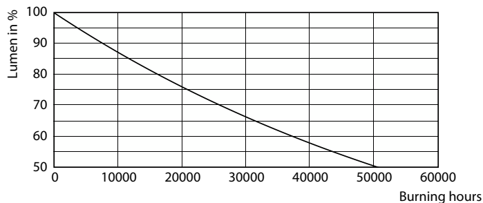
Lumen Maintenance Diagram - LEDspot 50W PAR20 827 100-240V 25D ND SO
