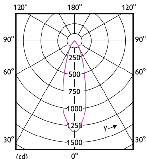
Light Distribution Diagram - LEDspot 50W PAR20 827 100-240V 25D ND SO
