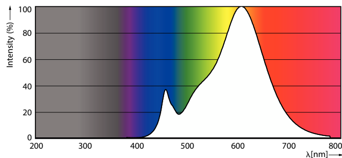
Spectral Power Distribution Colour - LEDspot 50W PAR20 827 100-240V 25D ND SO
