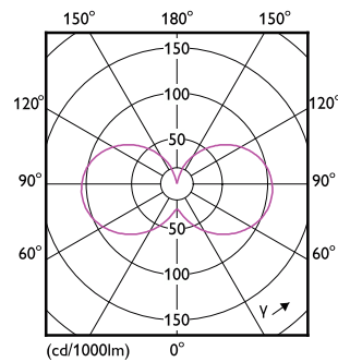
Light Distribution Diagram - LEDCapsule 40W G9 865 WV ND
