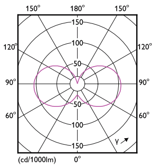
Light Distribution Diagram - LEDCapsule 40W G9 827 WV ND
