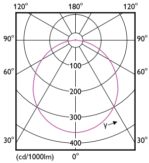
Light Distribution Diagram - DL252 G2 R SQ LED 2000 40K 24W 11" WW
