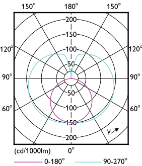
Light Distribution Diagram - MAS LEDtube VLE 1500mm HO 19W 840 T8 BR
