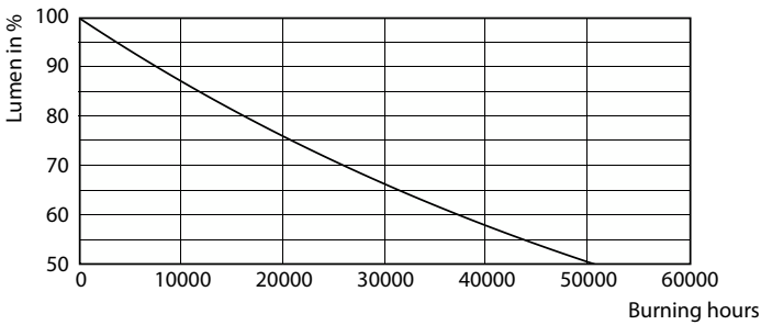
Lumen Maintenance Diagram - MAS LEDtube VLE 1500mm HO 19W 840 T8 BR
