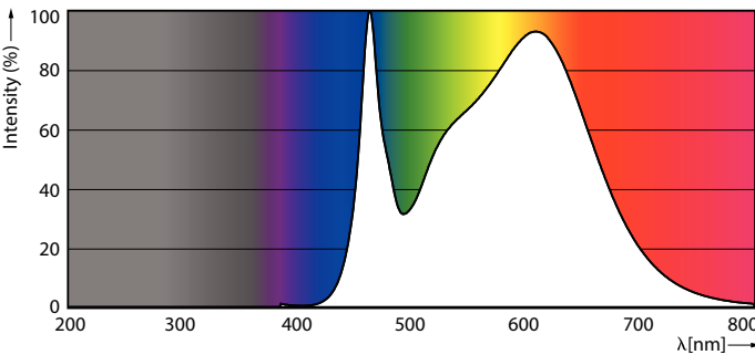
Spectral Power Distribution Colour - MAS LEDtube VLE 1500mm HO 19W 840 T8 BR
