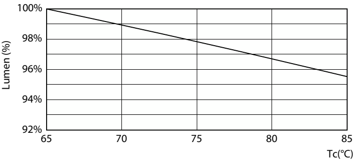
Lumen Maintenance Diagram - MAS LEDtube VLE 1500mm HO 19W 840 T8 BR
