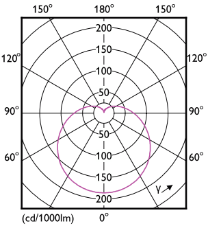
Light Distribution Diagram - LEDBulb 9W E27 4000K W 1PF/40 BR
