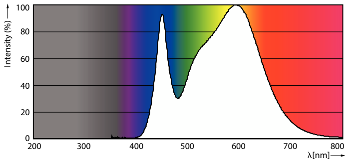
Spectral Power Distribution Colour - LEDBulb 9W E27 4000K W 1PF/40 BR
