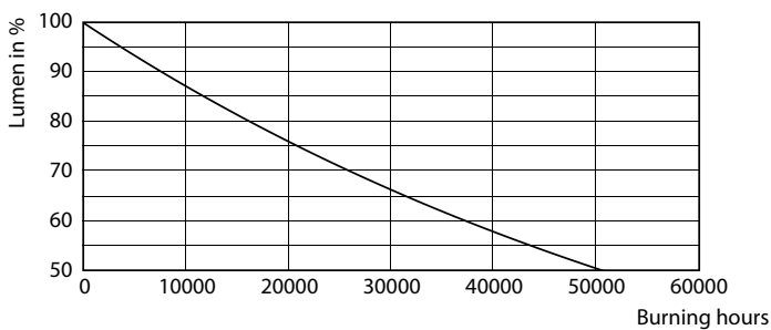
Lumen Maintenance Diagram - LEDBulb 9W E27 4000K W 1PF/40 BR
