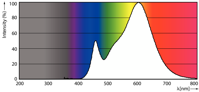
Spectral Power Distribution Colour - LEDBulb 9W E27 3000K W 1PF/40 BR
