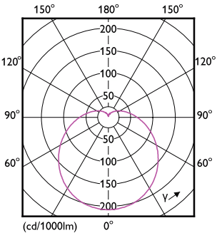
Light Distribution Diagram - LEDBulb 9W E27 3000K W 1PF/40 BR
