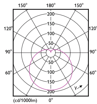
Light Distribution Diagram - LEDBulb 7W E27 6500K W 1PF/40 BR
