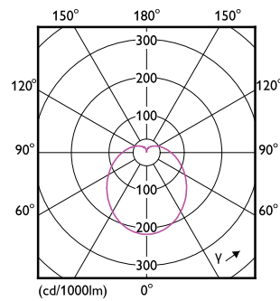
Light Distribution Diagram - LEDBulb 7W E27 3000K W 1PF/40 BR
