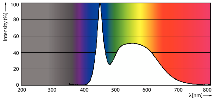
Spectral Power Distribution Colour - LEDBulb 4.5W E27 6500K W 1PF/40 BR
