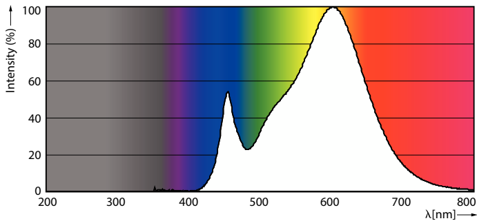
Spectral Power Distribution Colour - LEDBulb 4W E27 3000K 100-240VG45 BR
