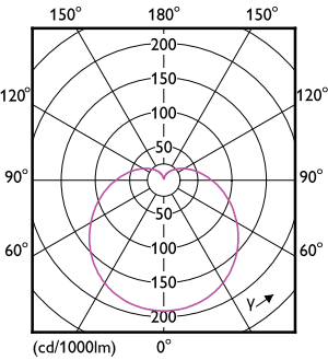
Light Distribution Diagram - LEDBulb 4W E27 3000K 100-240VG45 BR
