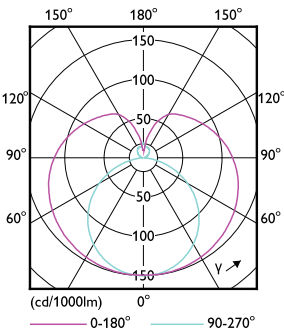
Light Distribution Diagram - CorePro LEDtube 600mm 9W 865 T8 C W G
