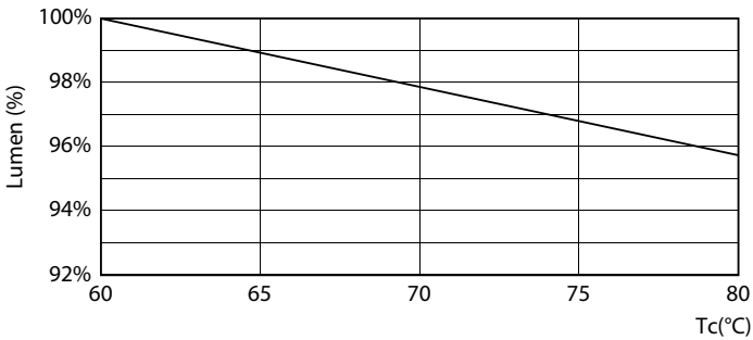
Lumen Maintenance Diagram - CorePro LEDtube 600mm 9W 865 T8 C W G
