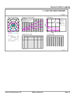
General uniform lighting - CorePro LEDtube 1200mm HO 18W865 C W G
