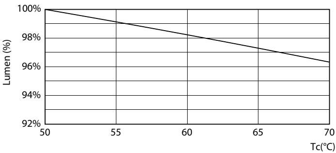
Lumen Maintenance Diagram - CorePro LEDtube 600mm 8W865 G5 I BR
