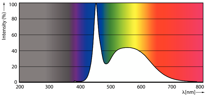
Spectral Power Distribution Colour - CorePro LEDtube 600mm 8W865 G5 I BR
