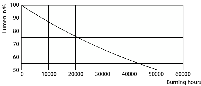
Lumen Maintenance Diagram - CorePro LEDtube 600mm 8W865 G5 I BR
