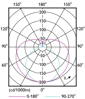
Light Distribution Diagram - CorePro LEDtube 600mm 8W865 G5 I BR
