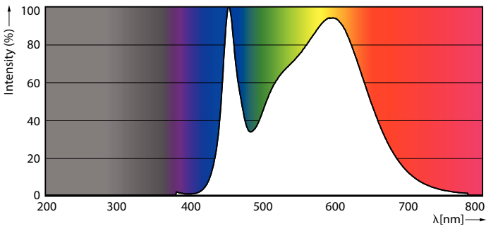
Spectral Power Distribution Colour - CorePro LEDtube 600mm 8W840 G5 I BR
