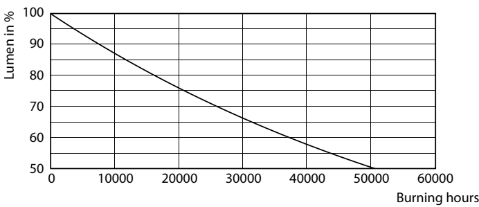
Lumen Maintenance Diagram - CorePro LEDtube 600mm 8W830 G5 I BR
