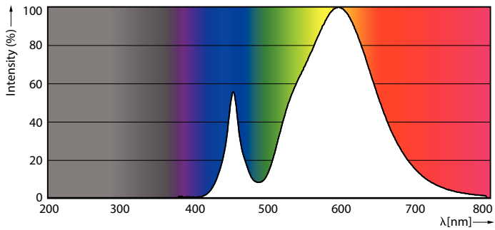
Spectral Power Distribution Colour - CorePro LEDtube 600mm 8W830 G5 I BR
