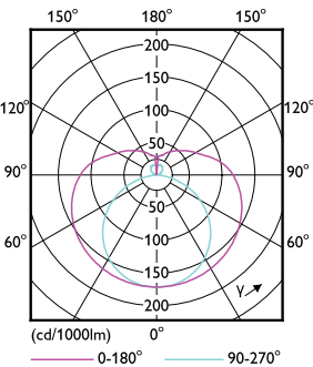
Light Distribution Diagram - CorePro LEDtube 600mm 8W830 G5 I BR
