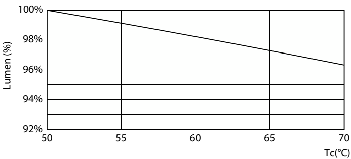
Lumen Maintenance Diagram - CorePro LEDtube 600mm 8W830 G5 I BR
