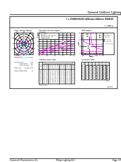
General uniform lighting - CorePro LEDtube 600mm 8W830 G5 I BR
