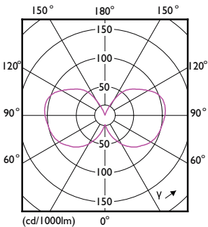
Light Distribution Diagram - LEDClassic 35W G93 E27 825 100-240 ND BR
