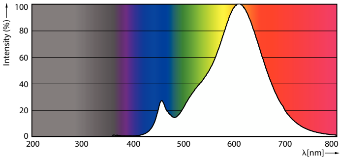
Spectral Power Distribution Colour - LEDClassic 35W G93 E27 825 100-240 ND BR
