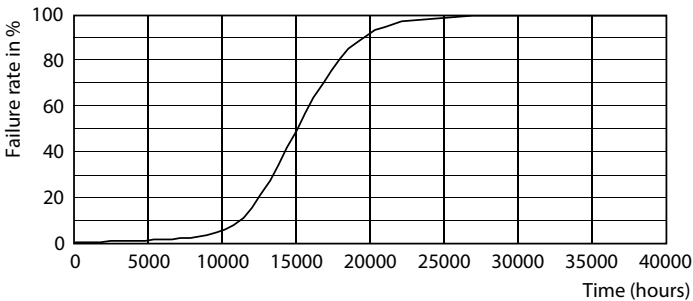
Life Expectancy Diagram - LEDClassic 35W A60 E27 825 100-240V NDBR
