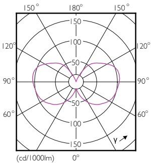
Light Distribution Diagram - LEDClassic 35W A60 E27 825 100-240V NDBR
